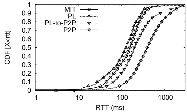
Figure 3: CDFs of latencies from different measurement platforms (semilog scale). Our measurement study exclusively between peers in Vuze (labeled P2P) exhibits double the median latency “in the wild” (labeled PL-to-P2P).
