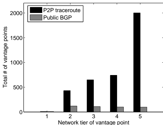
Figure 1: Number of vantage point ASes corresponding to inferred network tiers.
