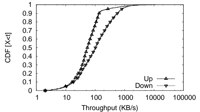
Figure 4: CDF of transfer rates for all users, where the median is only 50 to 100 KB/s. This suggests that the BitTorrent system is dominated by mid-to-low-capacity hosts.
