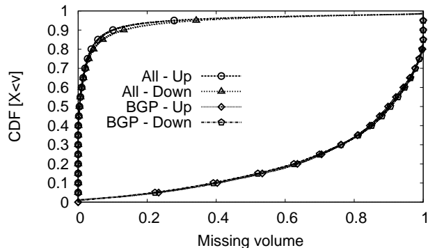
Figure 2: CDF of the portion of each host's traffic volume that could not be mapped to a path based on both public views and traceroutes between a subset of P2P users.
