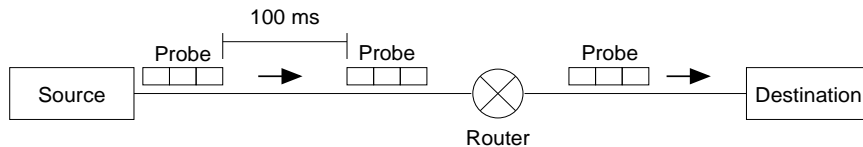
Figure 1: Measurement Methodology: The source sends a probe to the destination and waits 100 ms before sending the next probe. A probe consists of three packets, one of each protocol (ICMP, UDP, TCP), in a random order without spacing.
